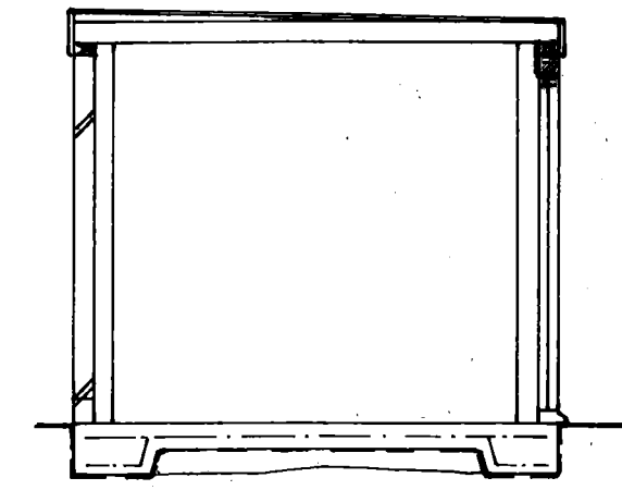
GARAGE SECTION 1:50
