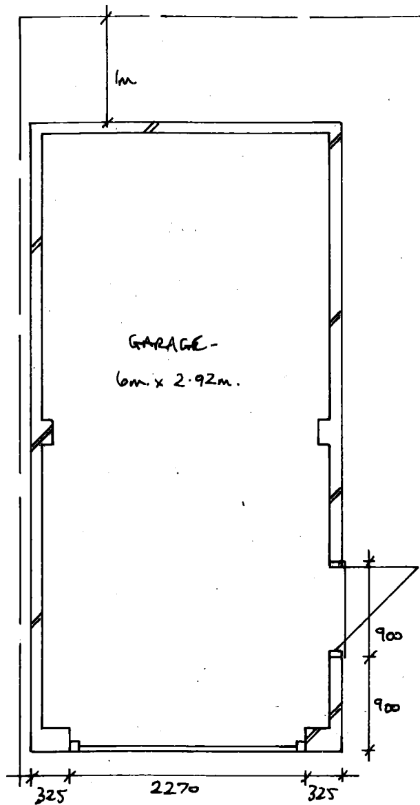
PROPOSED GARAGE PLAN 1:50
