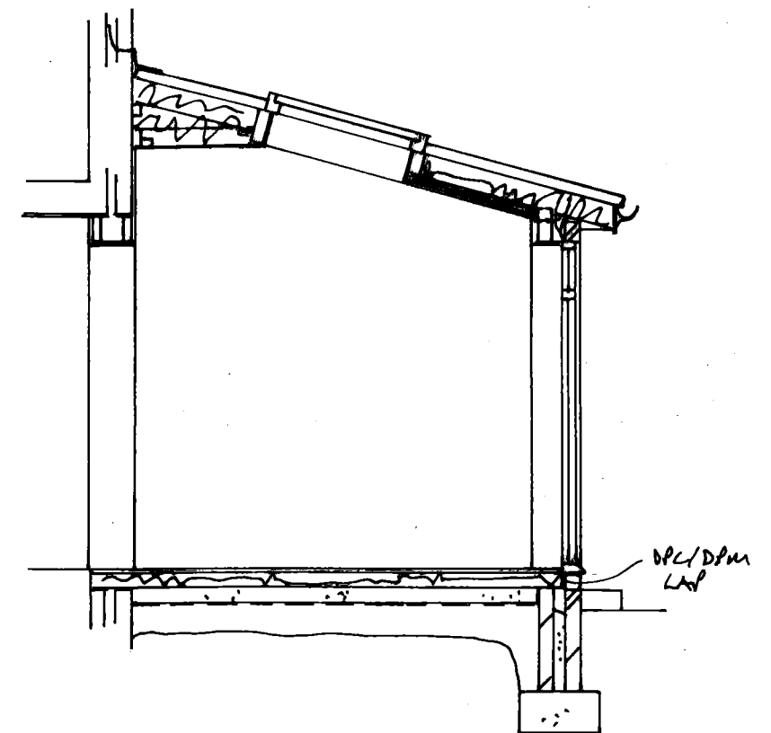
SECTION 1:50
